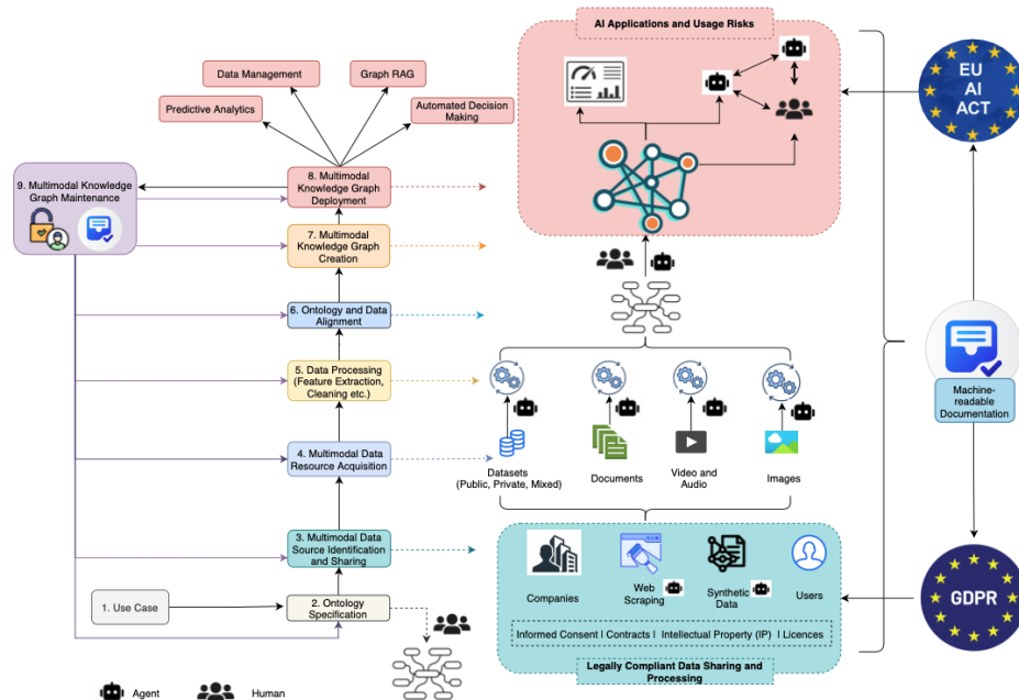
Figure 1: MMKGs' Development Example, Human and Agent Involvement, and Applicable Legislation. The process begins with defining a Use Case (1) and establishing an Ontology (2) , which feeds into Data Source Identification (3) and Resource Acquisition (4) . This data gathering is strictly governed by a legal framework covering informed consent, contracts, and intellectual property. The acquired multimodal data (datasets, documents, video, audio, images) undergo Data Processing (5) , Ontology Alignment (6) , are turned into a MMKG (7) . The MMKG Deployment (8) phase powers downstream AI applications such as Predictive Analytics, Graph RAG, and Automated Decision Making subject to the EU AI Act, all while undergoing continuous Maintenance (9) that needs to be carried out by authorised agents.
