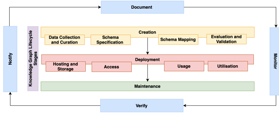
Figure 2: Knowledge Graph Lifecycle based on [40] and proposed Governance Mechanisms (in Blue)
